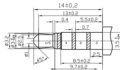
MATE PLUG
