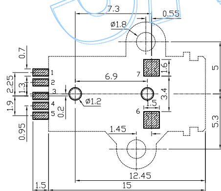
Recommended PAD Layout TOP VIEW
