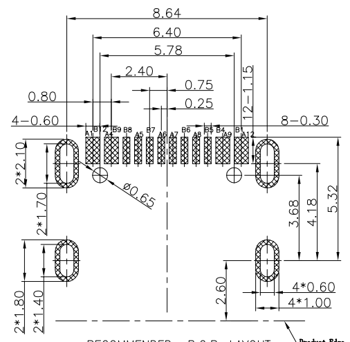
RECOMMENDED P.C.B. LAYOUT TOLERANCE UNSPECIFIED ±0.05mm
