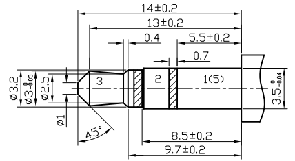
MATE PLUG
