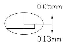
COPLANARITY
