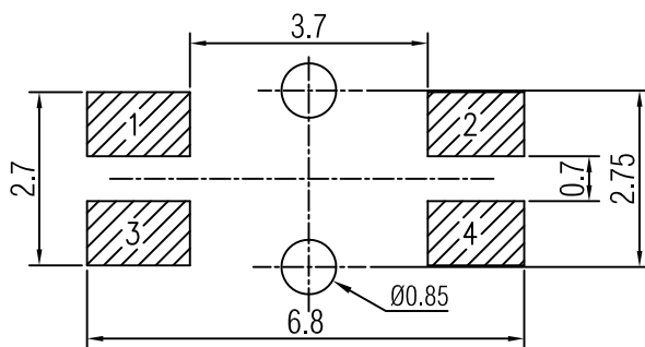
Recommended PAD Layout \Phi \pm 0.05 TOP VIEW
