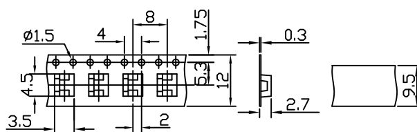
CARRIER TAPE
