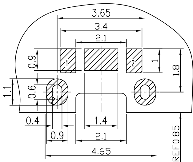
Recommended PAD Layout \Phi \pm 0.05 TOP VIEW
