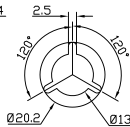
"A" DETAIL
