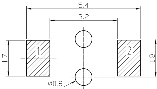
Recommended PAD Layout \oplus\pm 0.05 TOP VIEW
