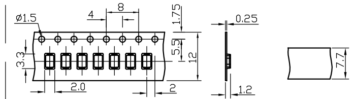
CARRIER TAPE
