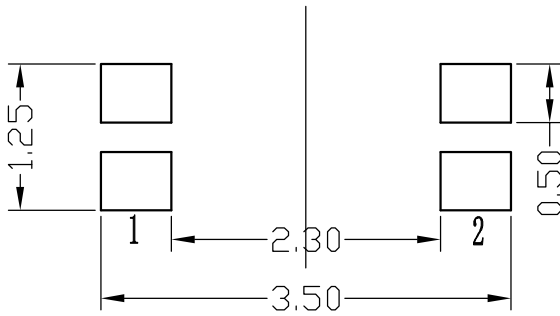
Recommended PAD Layout \pm 0.05
