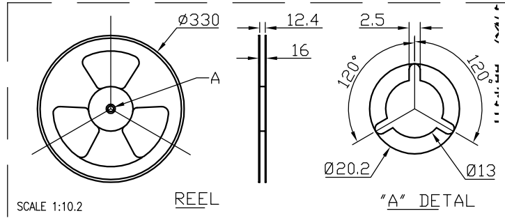
SCALE 1:10.2
