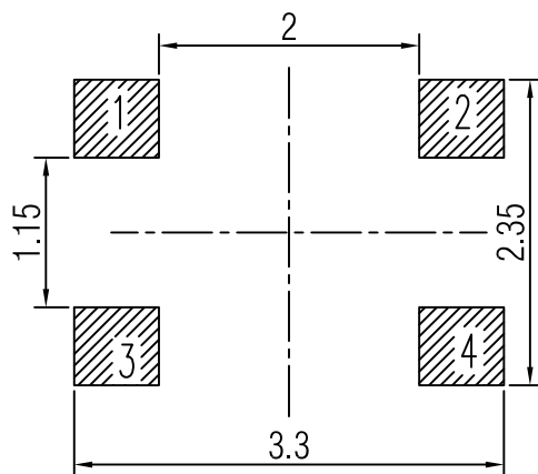
Recommended PAD Layout \Phi \pm 0.05 TOP VIEW
