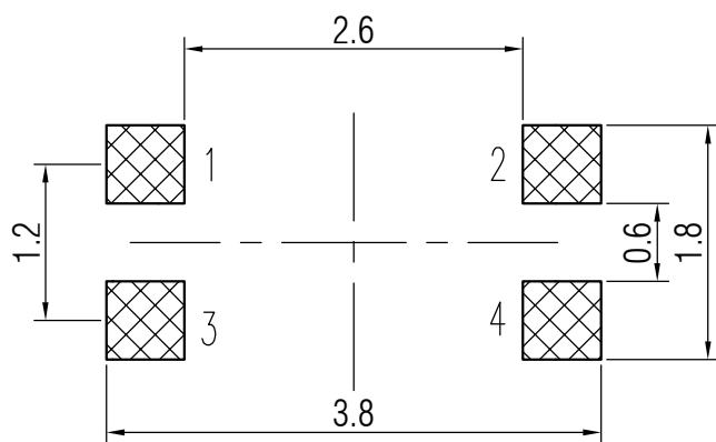
Recommended PAD Layout \Phi \pm 0.05 TOP VIEW
